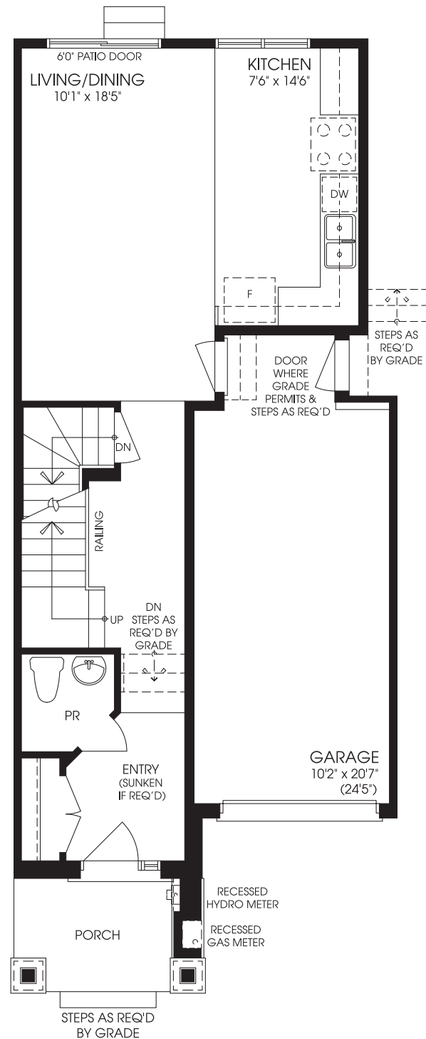
MAIN FLOOR ELEVATION 'A2'
