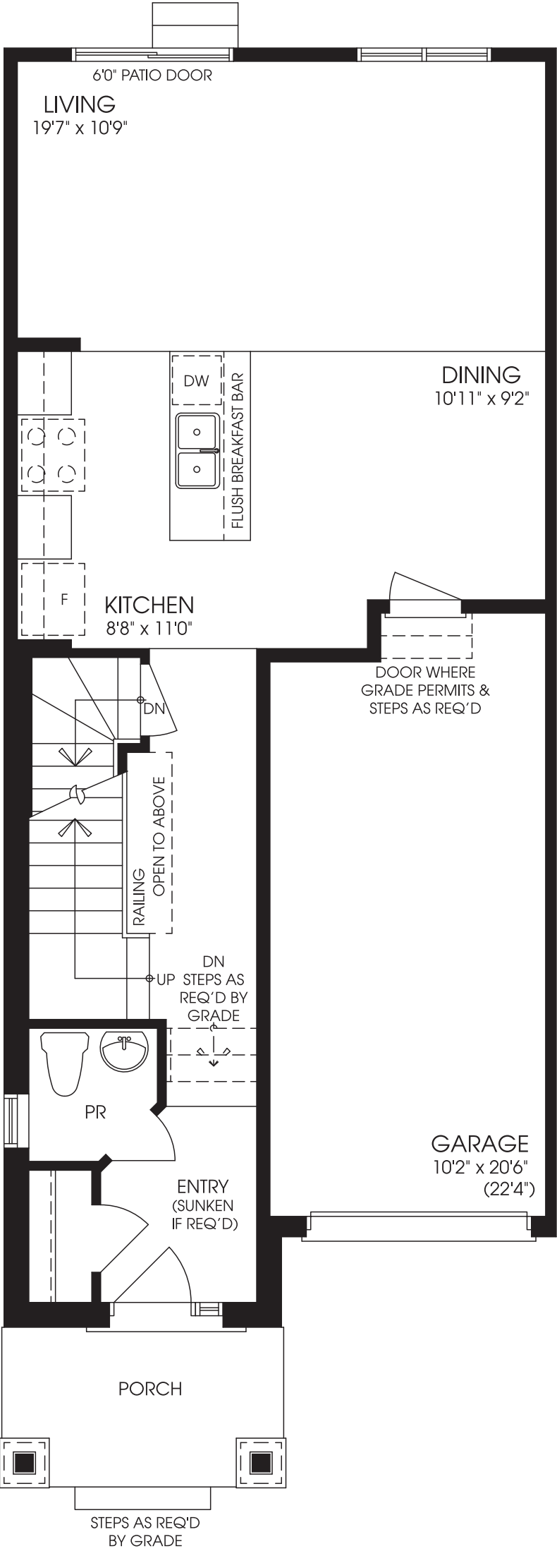
MAIN FLOOR ELEVATION 'A1'
