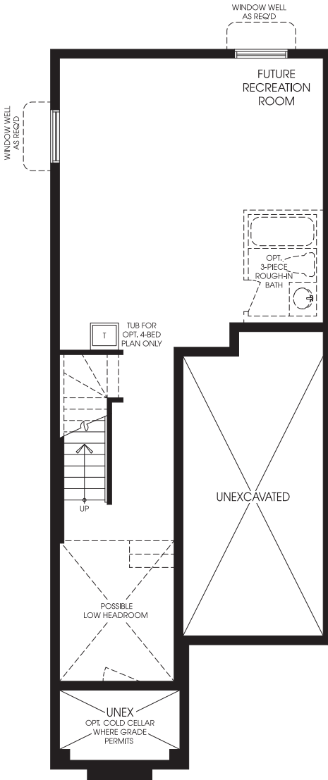
BASEMENT ELEVATION 'A1'
